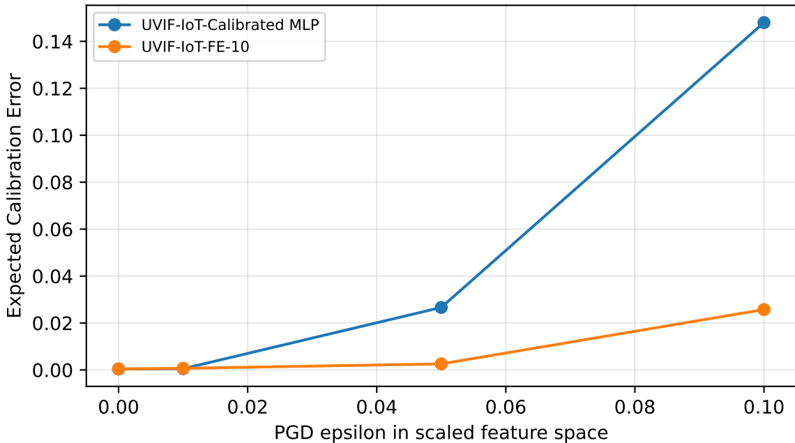
PGD Calibration on Test Subset
