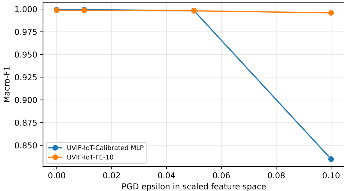
PGD Robustness on Test Subset
