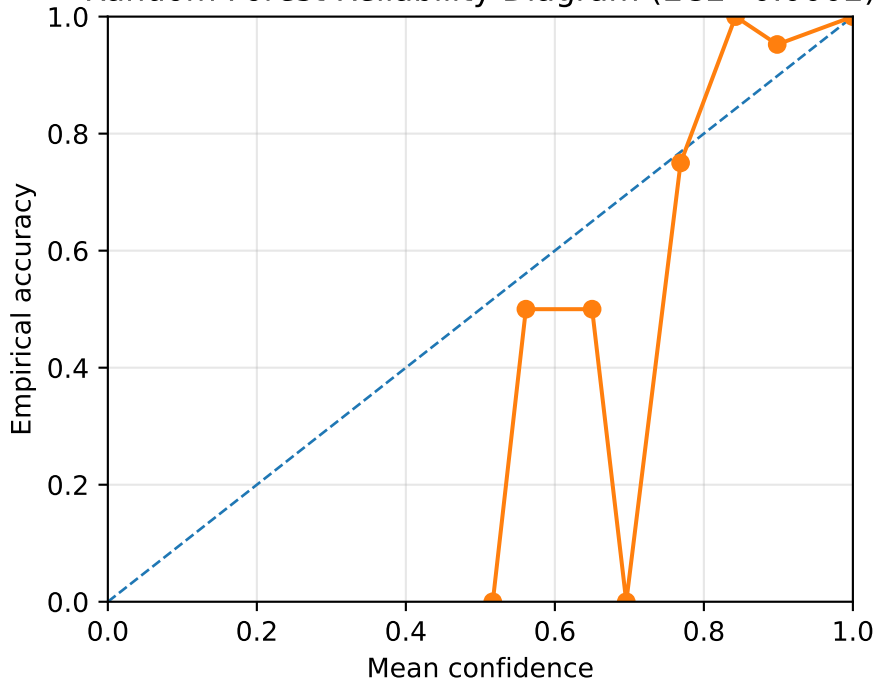
Random Forest Reliability Diagram (ECE=0.0002)
