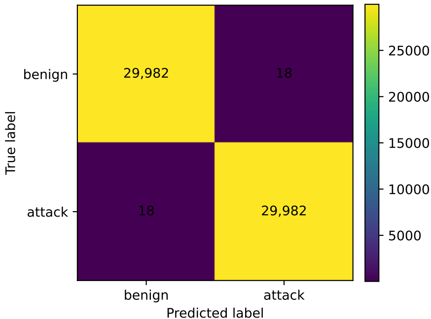
Standard MLP Confusion Matrix
