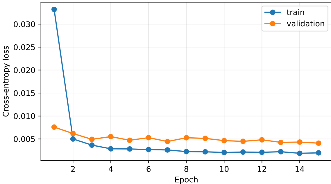
Standard MLP Training Curve
