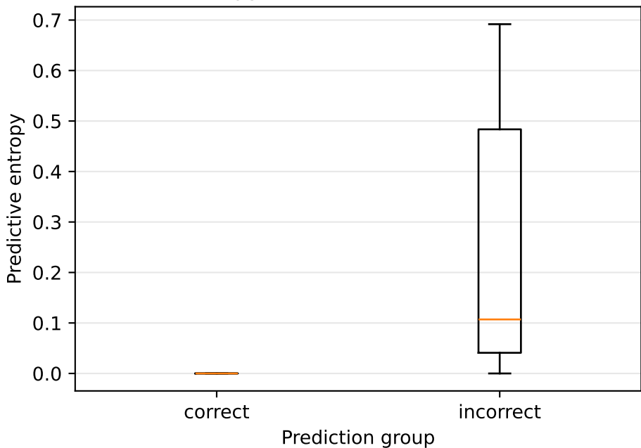
Predictive Entropy for Correct vs Incorrect Predictions
