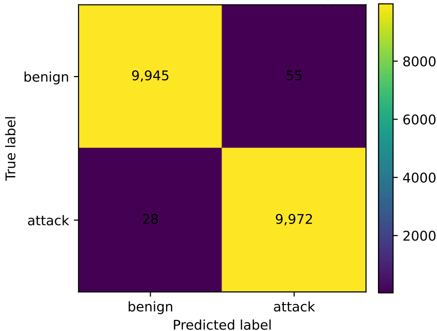
Feature-Efficient UVIF-IoT PGD CM, epsilon=0.1
