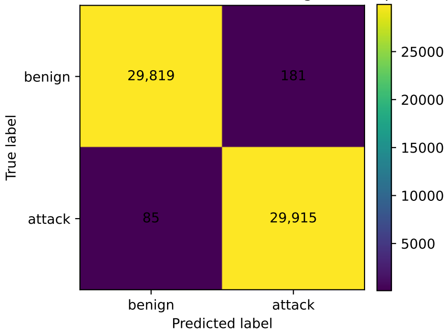
Feature-Efficient UVIF-IoT FGSM CM, budget=10, epsilon=0.1
