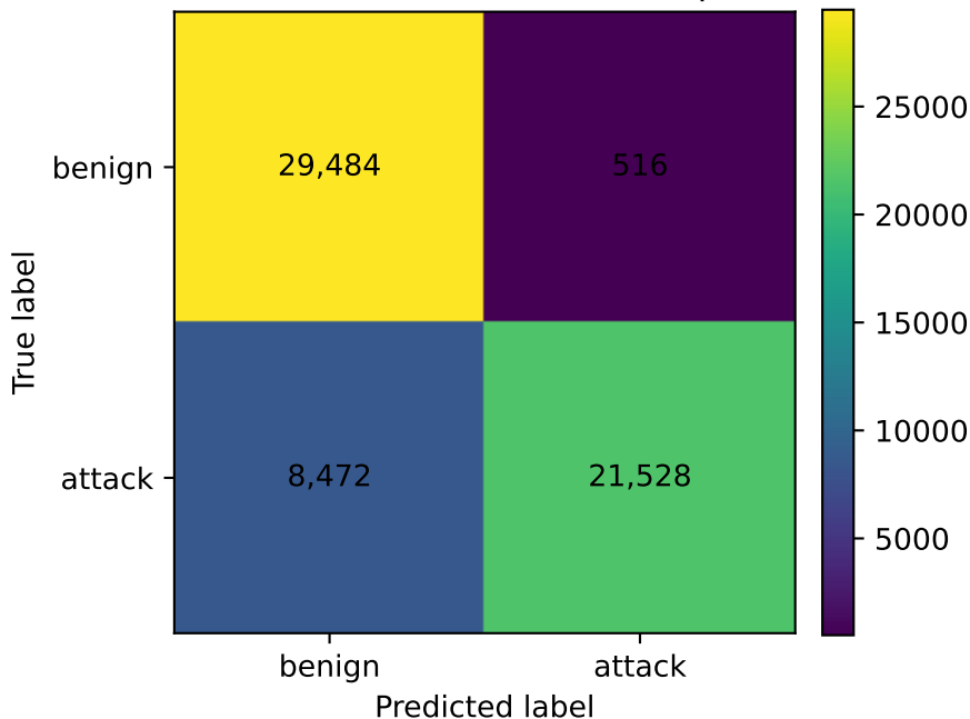
UVIF-IoT FGSM Confusion Matrix, epsilon=0.1
