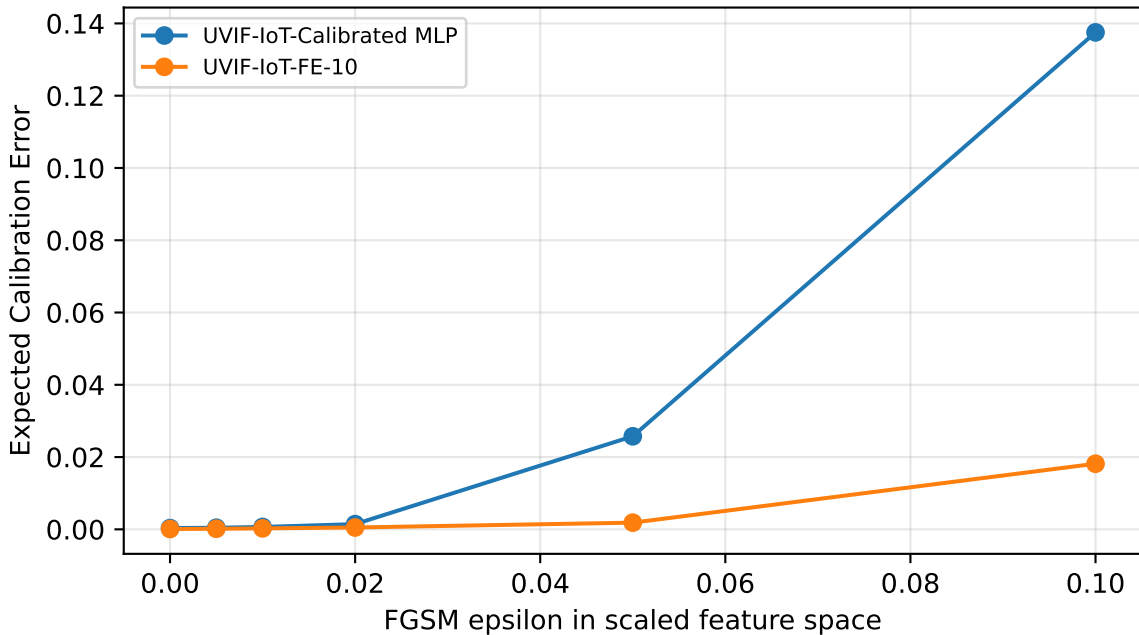
FGSM Calibration: Full vs Feature-Efficient UVIF-IoT
