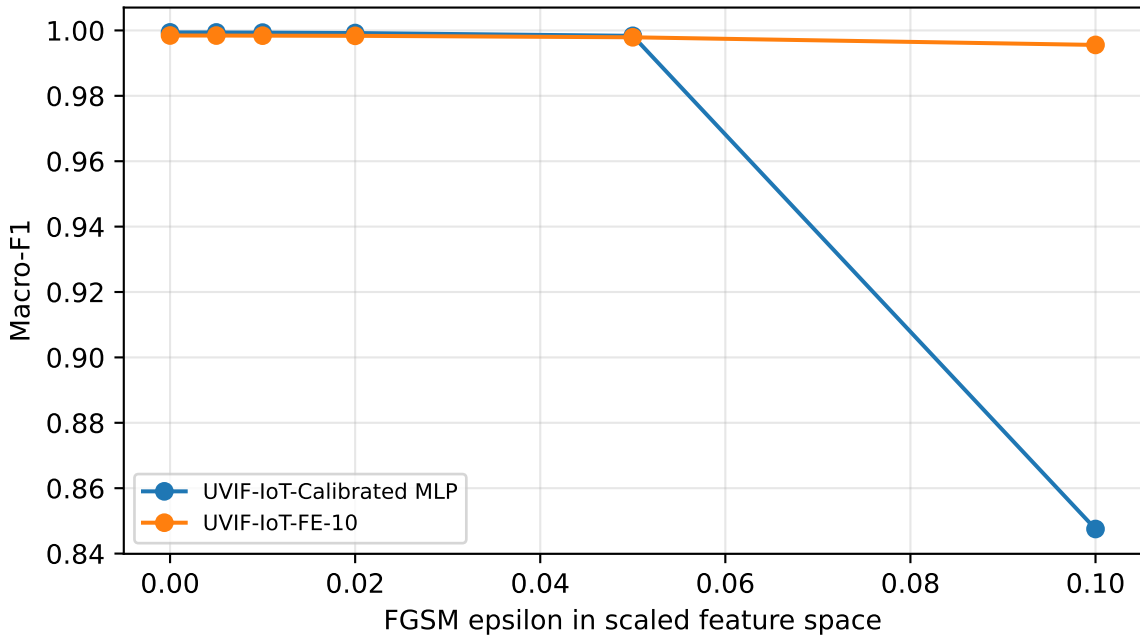
FGSM Robustness: Full vs Feature-Efficient UVIF-IoT
