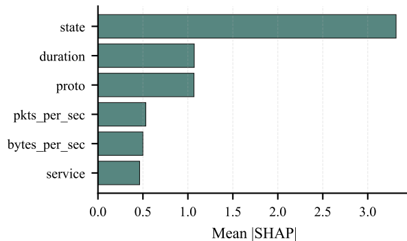
(b) Global SHAP: ToN-IoT
