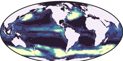
c. CbPM
