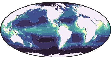
e. VGPM-Eppley
