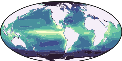
e. VGPM-Eppley
