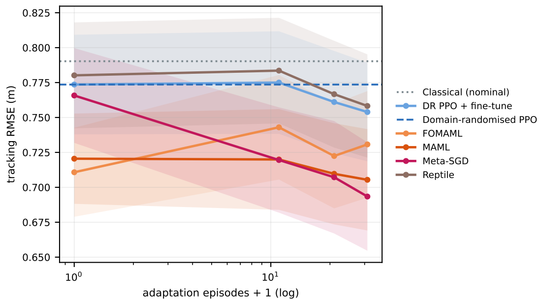
out-of-distribution tasks
