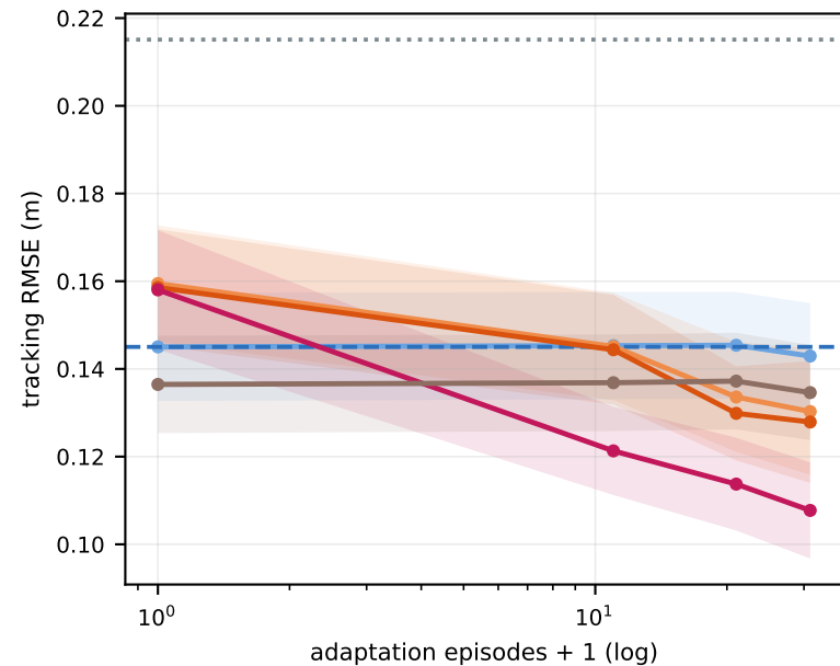
held-out tasks
