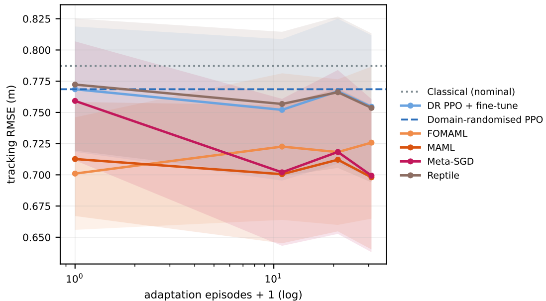
out-of-distribution tasks
