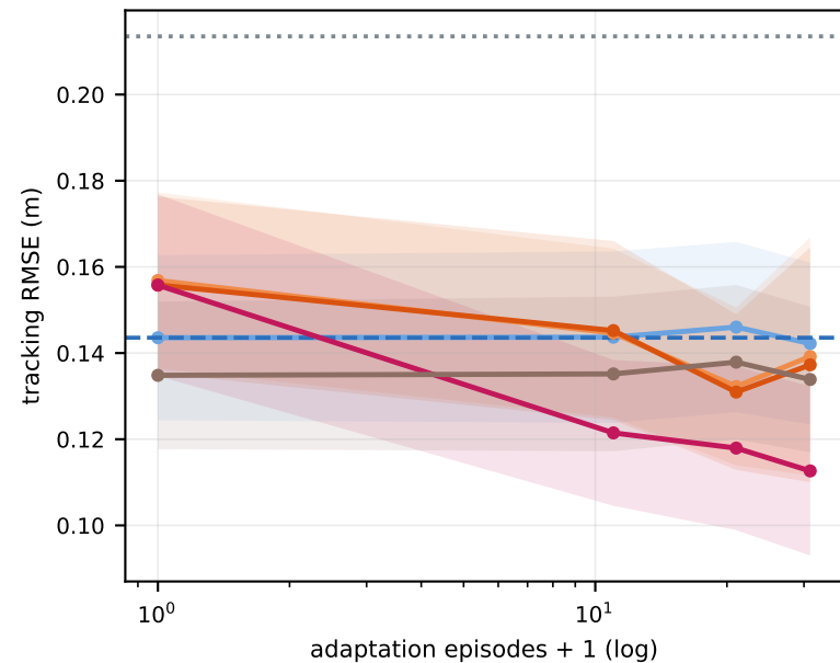
held-out tasks
