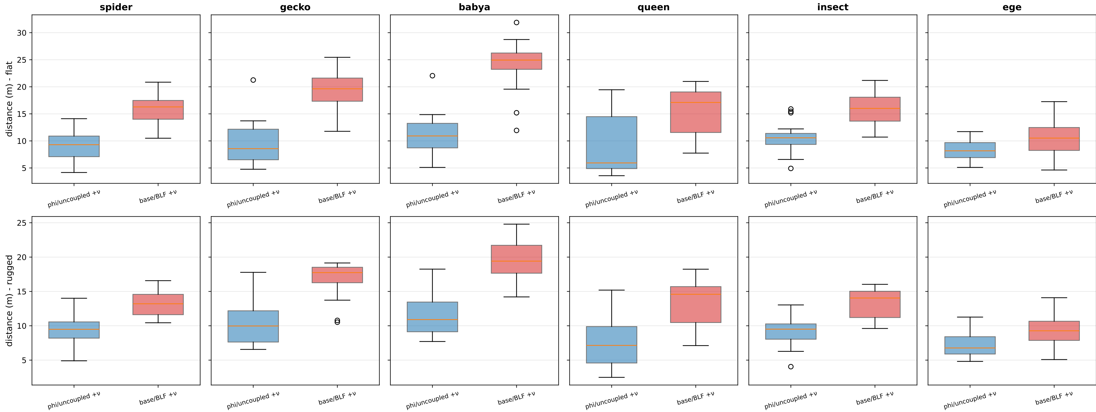
distance (m) per seed - phi+v vs BLF+v, flat &amp; rugged (n=30)
