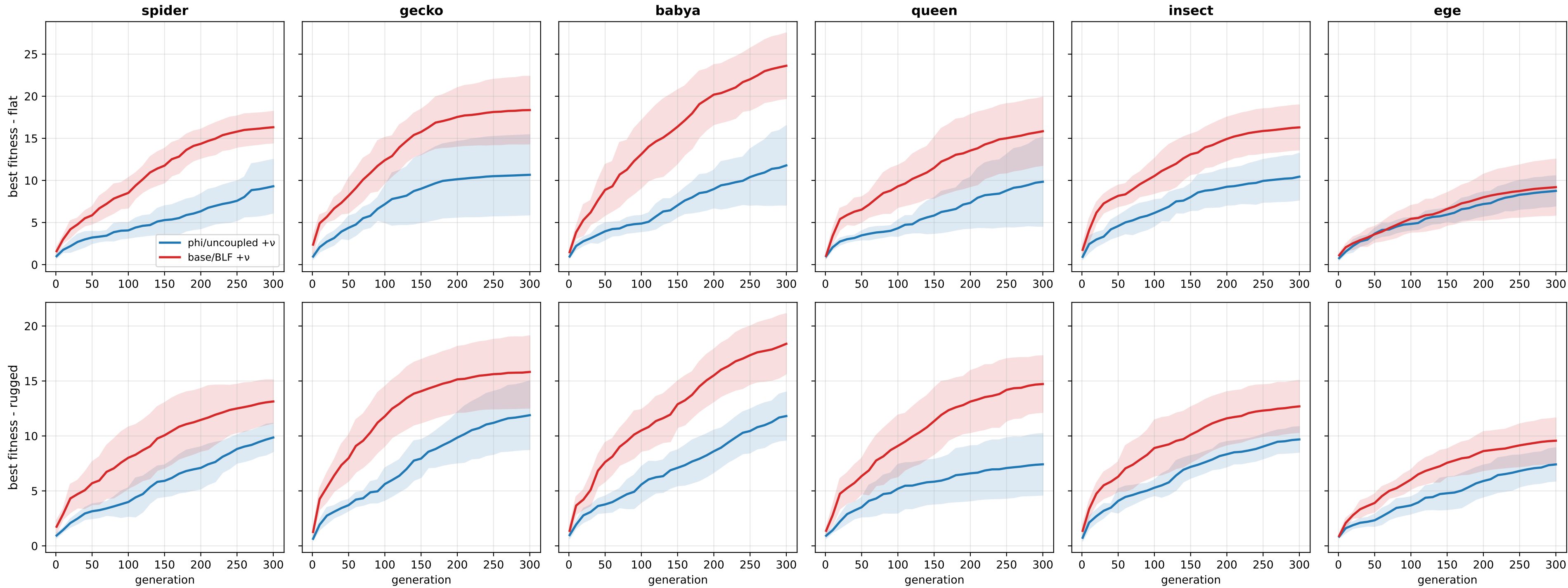
Convergence (mean \pm 1 std across 10 seeds), evolve_v, flat & rugged
