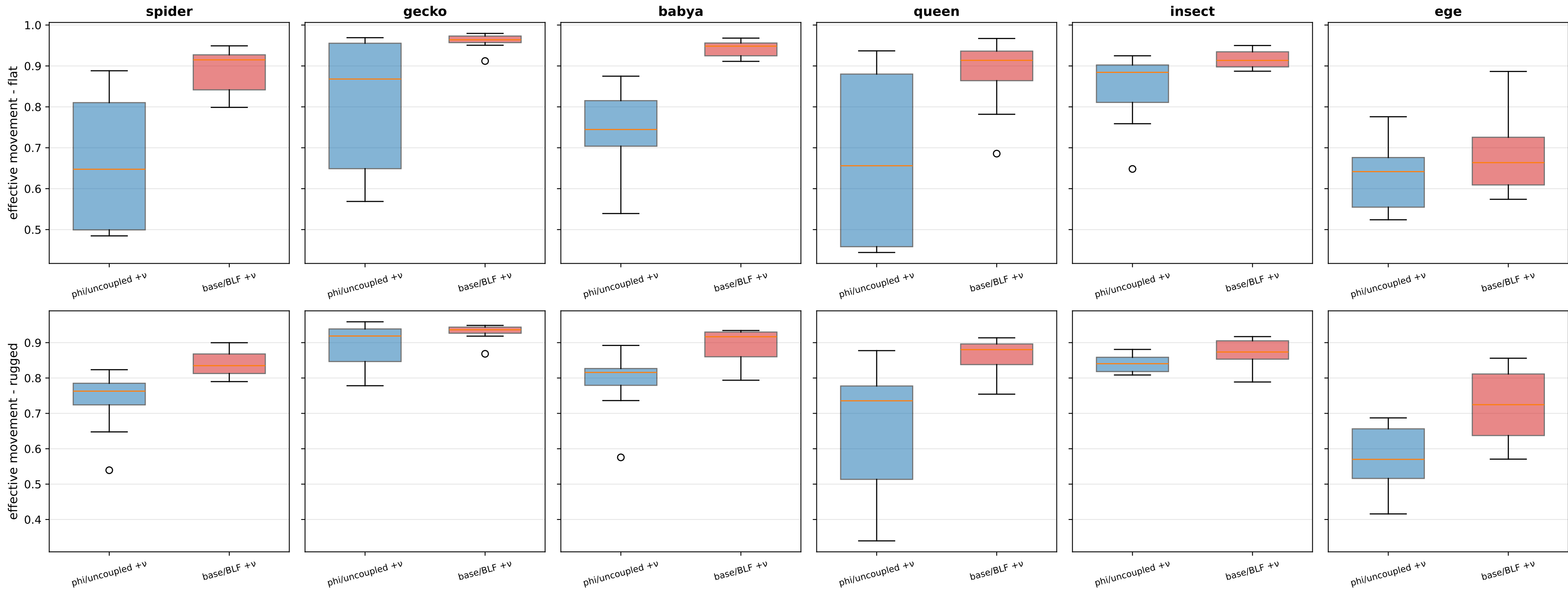
effective movement per seed - phi+v vs BLF+v, flat & rugged (n=10)
