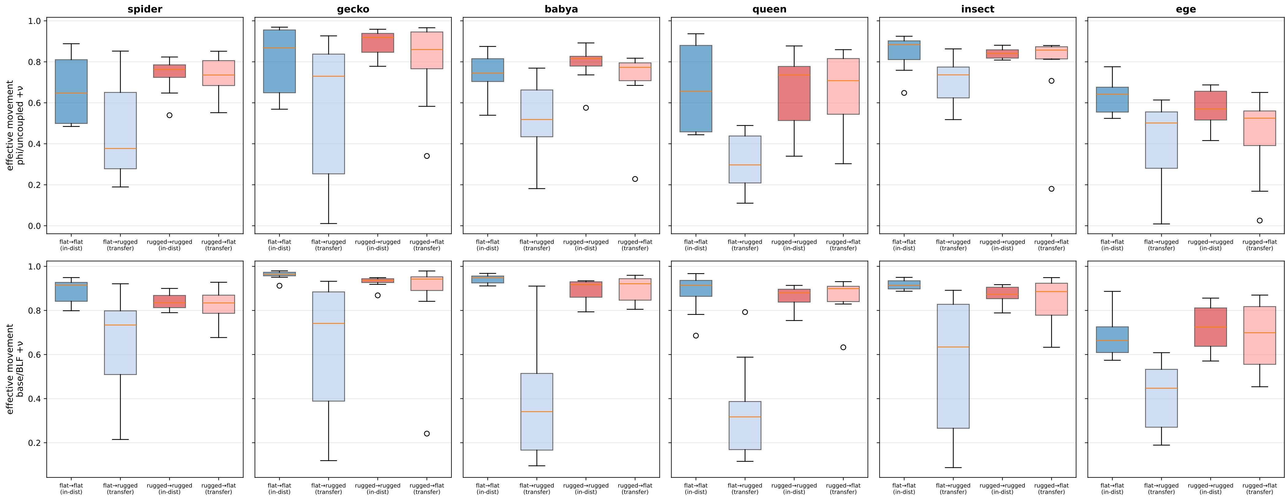
Cross-terrain transfer (evolve_v, effective movement, n=10)
