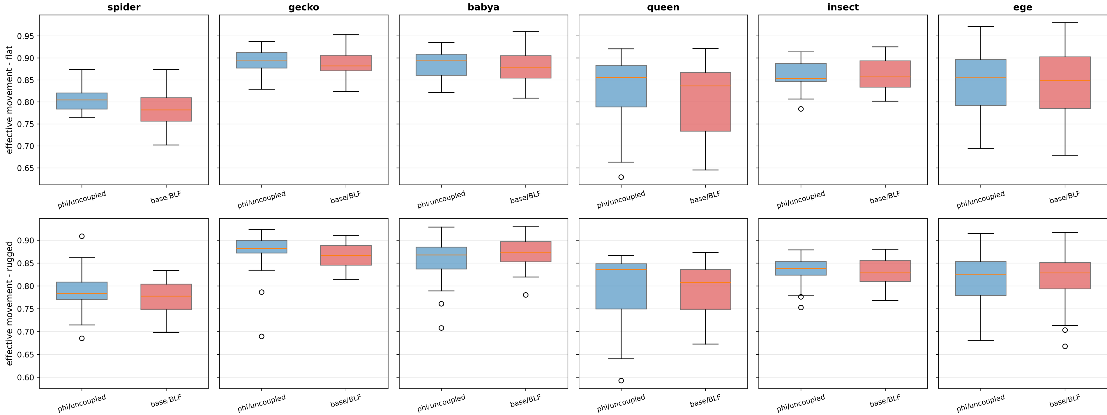
effective movement per seed - phi/uncoupled vs base/BLF, flat & rugged (n=30 each)
