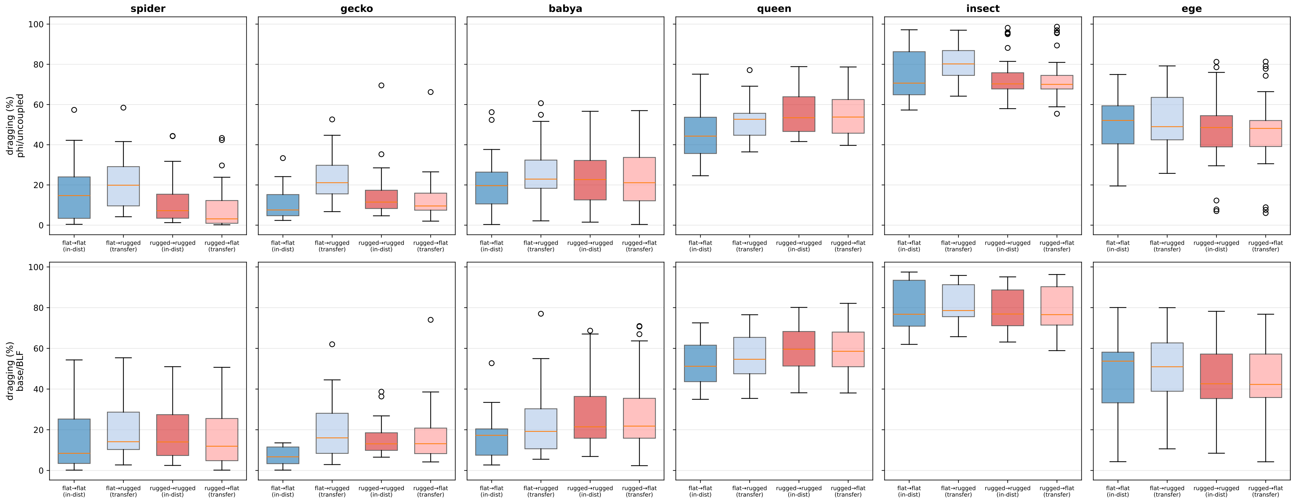
Cross-terrain transfer (dragging (%), n=30 each)
