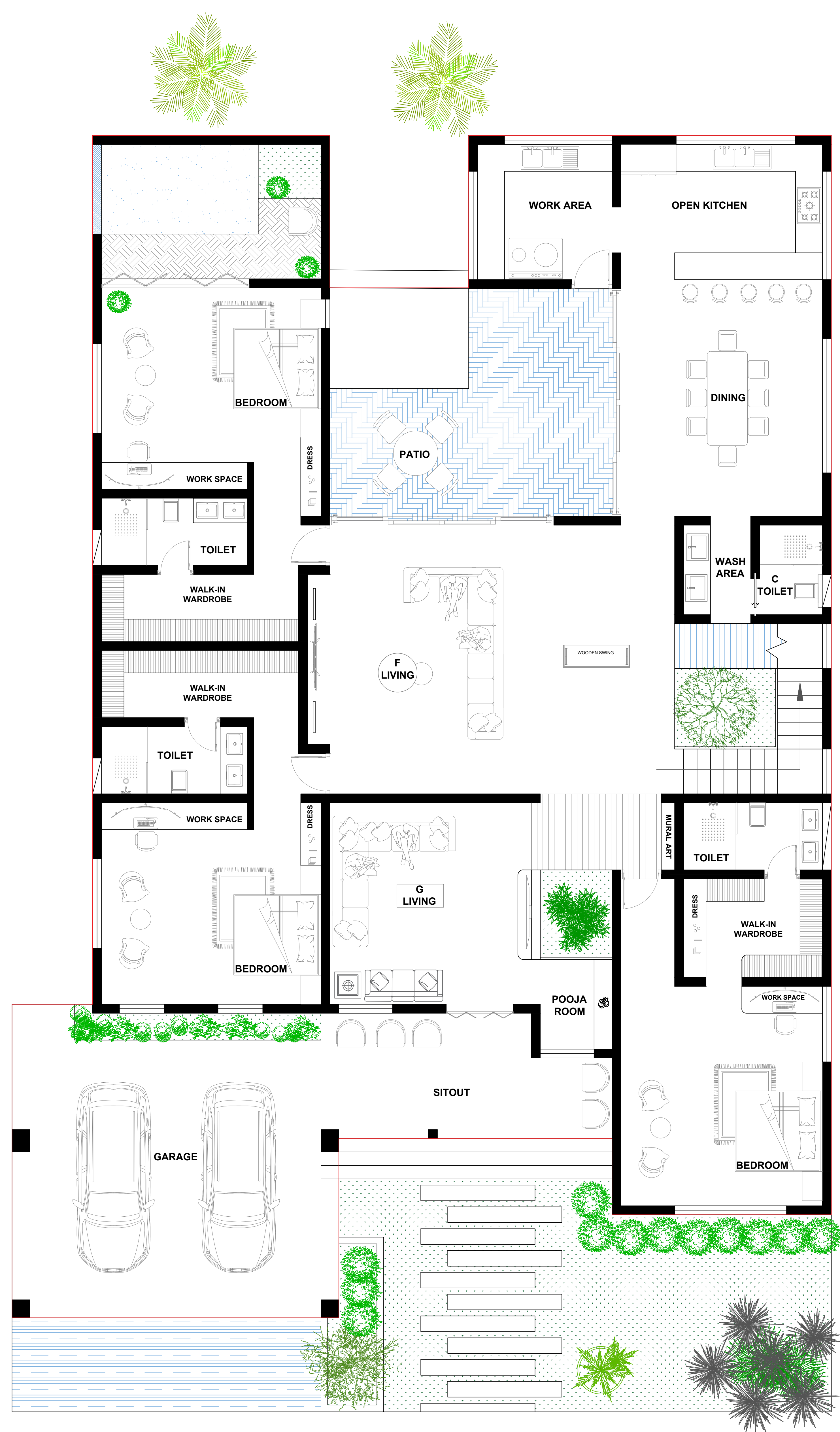
GROUND FLOOR AREA - 4326 SQFT
