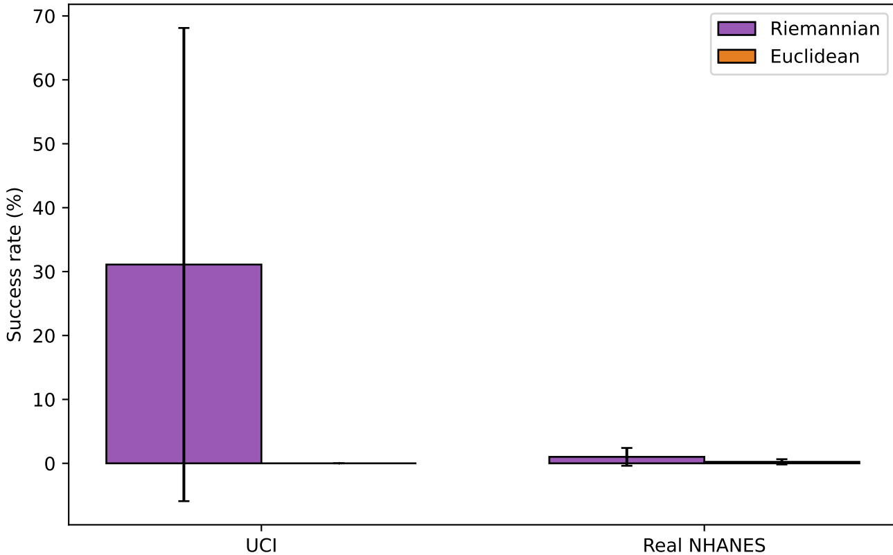
Fig 3 — Riemannian vs. Euclidean under EGD: REVERSES every prior session's null finding (mechanism: Euclidean favors shorter paths; EGD's guarantee accumulates change per hop, so path length now matters)
