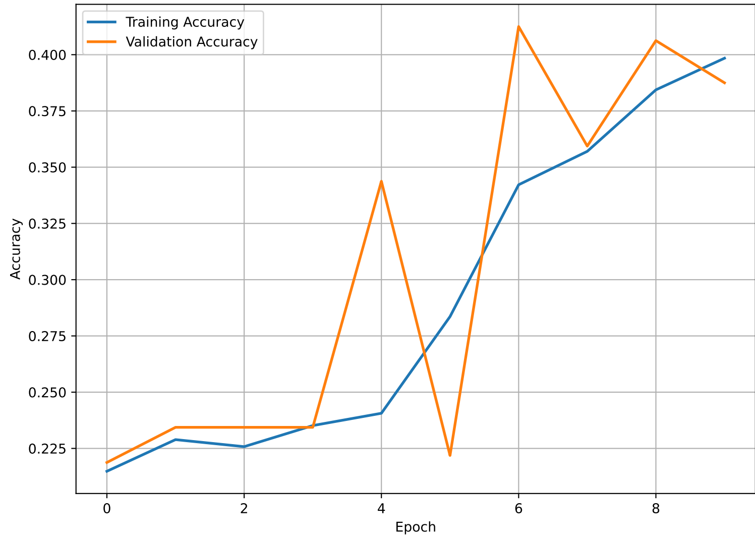
Custom CNN Accuracy
