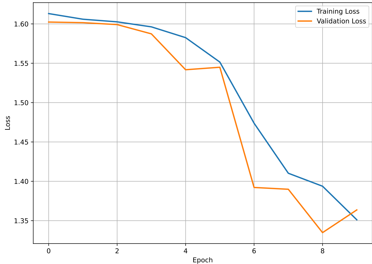
Custom CNN Loss
