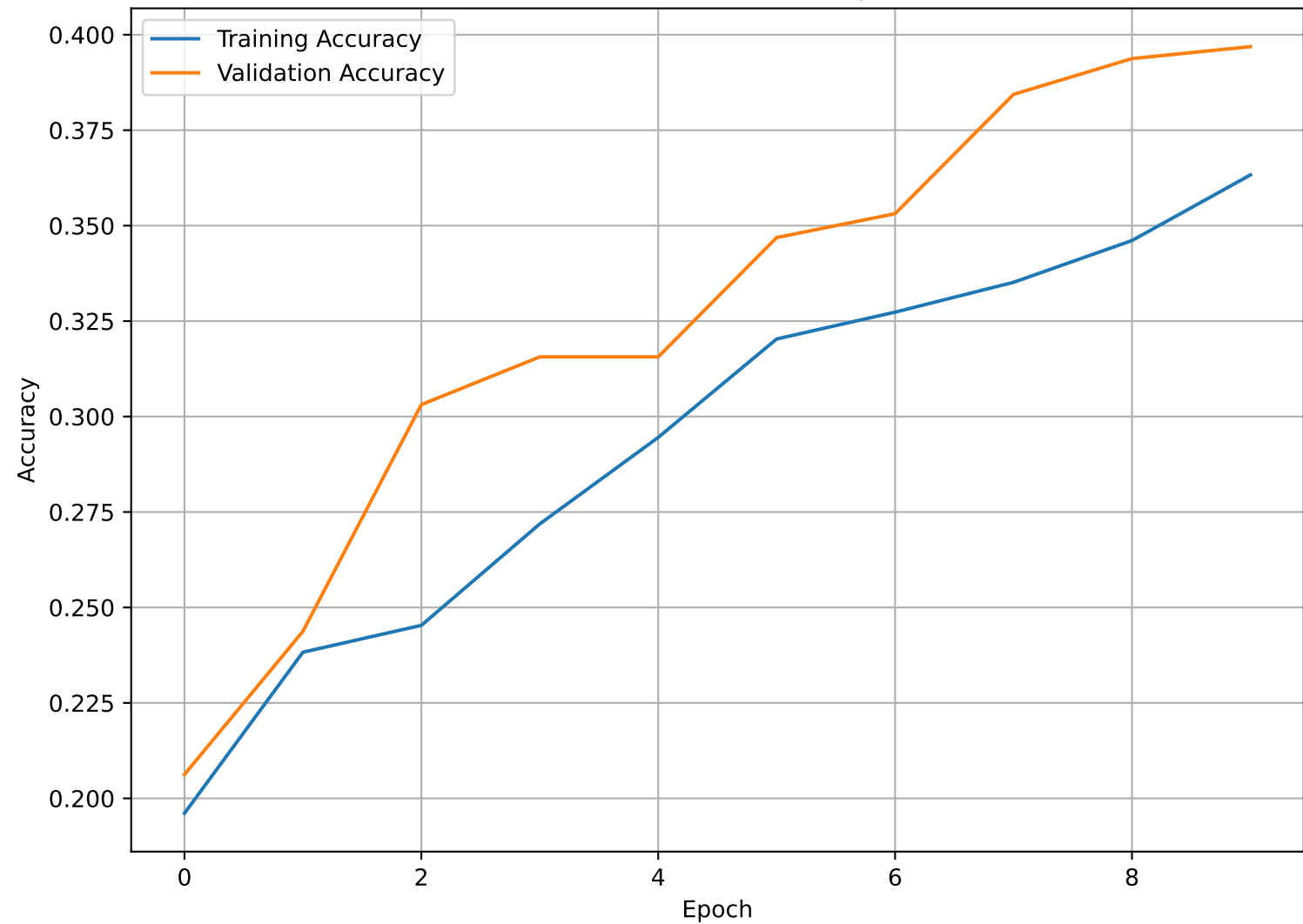
MobileNetV2 Accuracy
