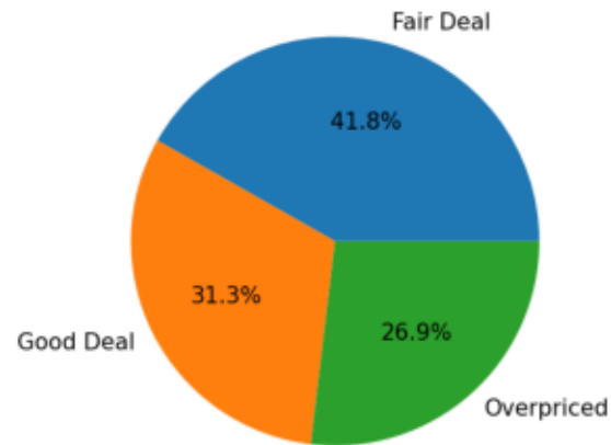
Deal Mix
