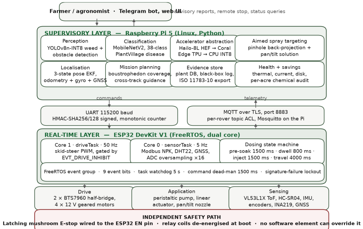
Figure 1. Three-tier system architecture. The horizontal rule between the Raspberry Pi 5 and the ESP32 is the real-time boundary: everything below it is hard real-time and safety-relevant, everything above it is soft real-time and may be preempted, delayed or restarted without compromising machine safety. The independent safety path at the base is electrically outside both tiers.
