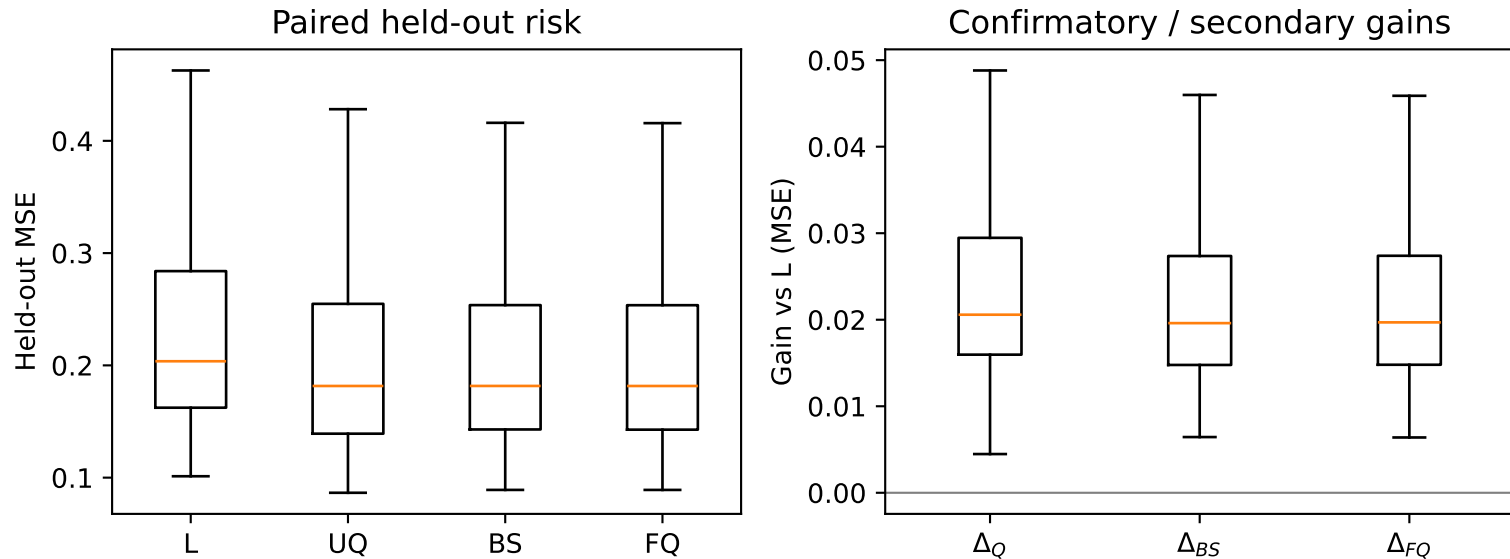
Figure 1 — primary and secondary held-out risk (frozen QLCA)
