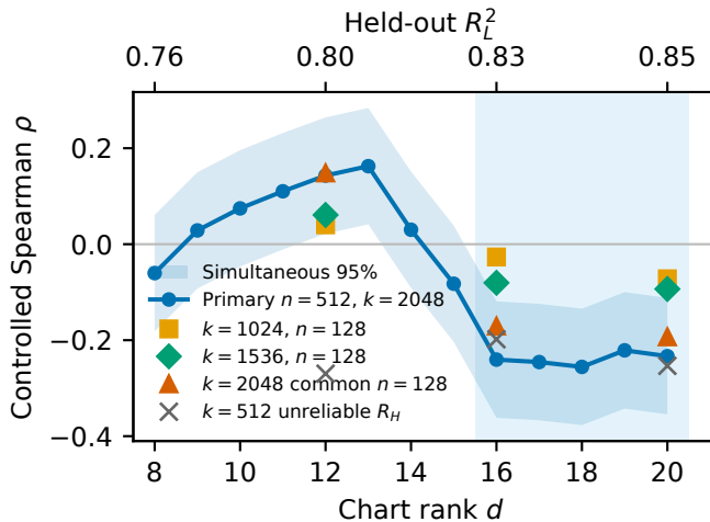
Controlled \rho(K_H^{\text{cross}}, R_{\text{local}}^2)
