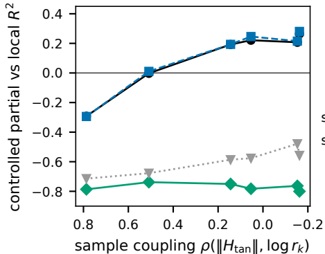
(a) known surface, intrinsic-linear label
