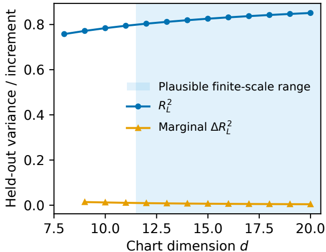
Adequacy, not an eigengap
