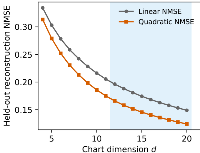
Held-out reconstruction error
