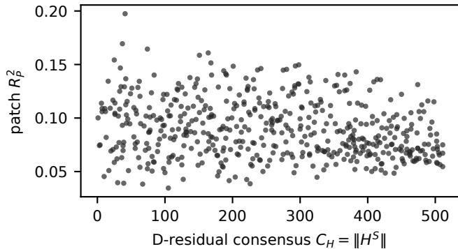
frozen probe outcome vs D-residual
