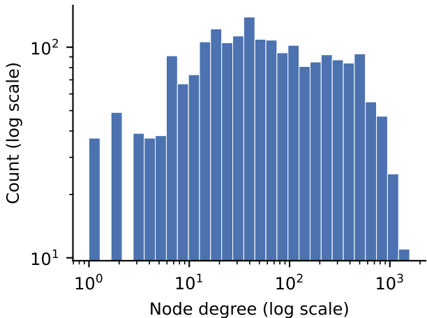
Degree distribution
