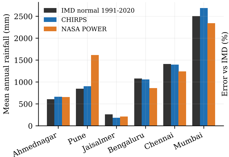
(a) Mean annual rainfall
