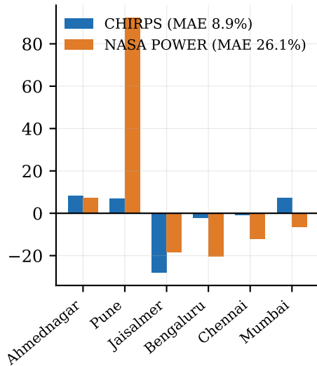
(b) Relative error
