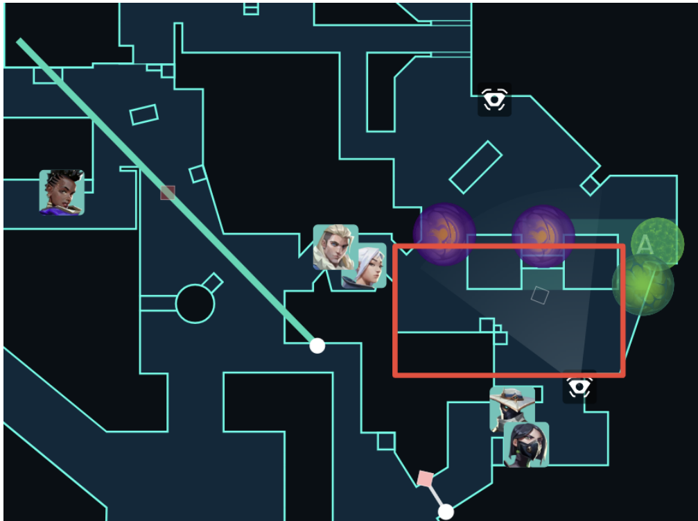
Figure 8: A2 Execute
