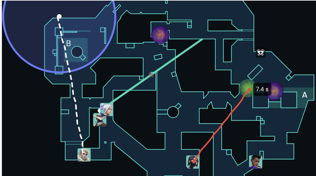
Figure 10: A3 Execute
