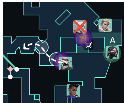
Figure 6: A1 Execute
