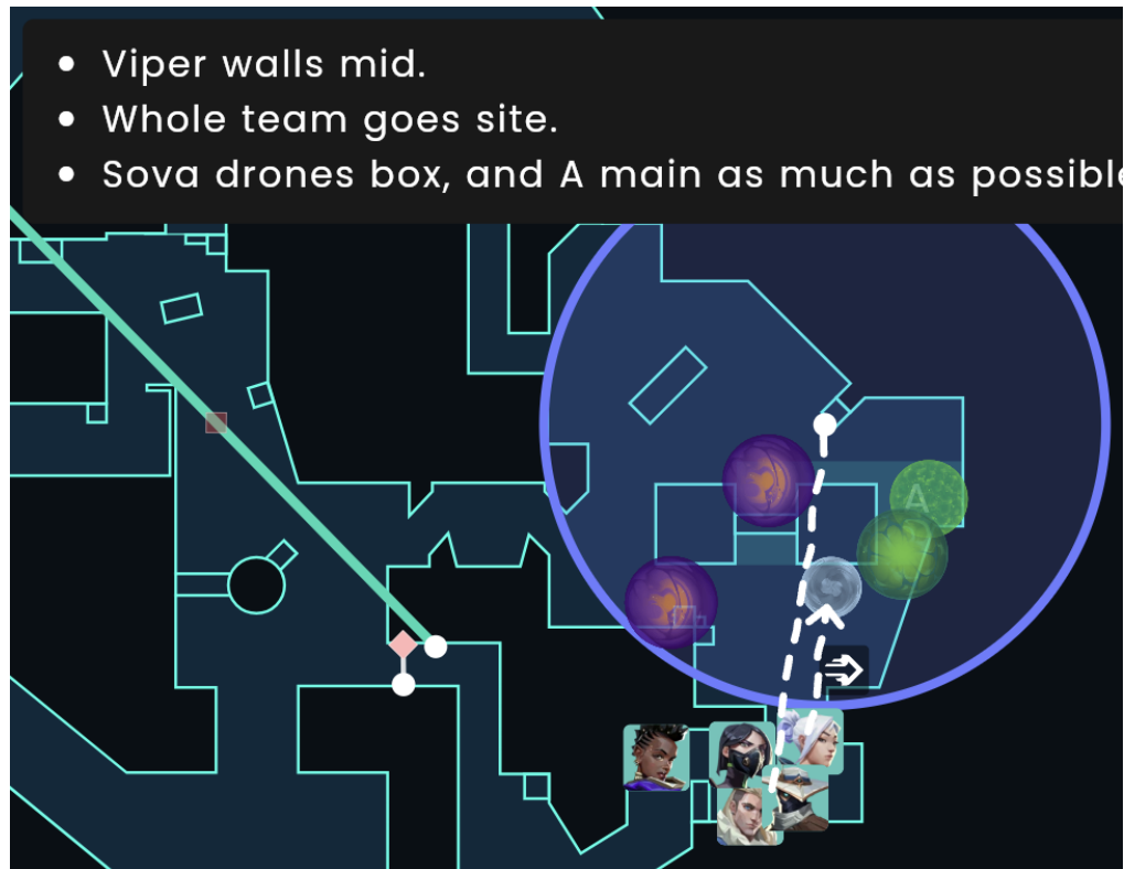
Figure 5: A1 Execute
