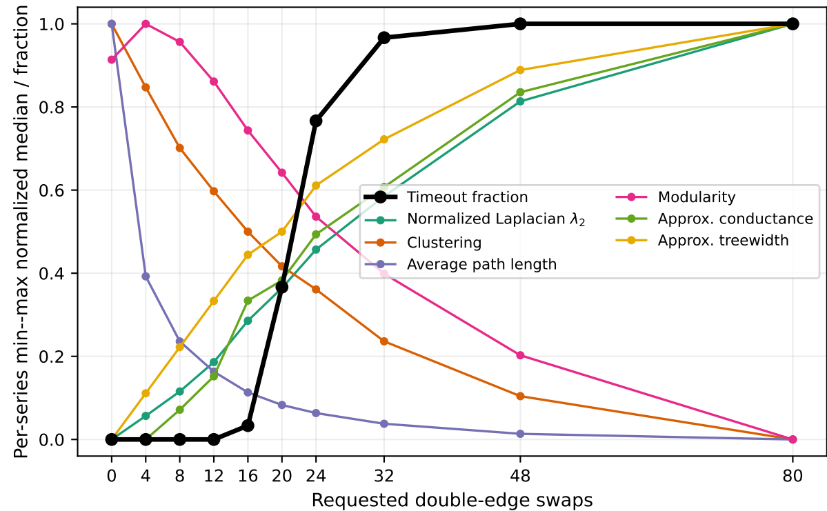
Descriptive comparison; normalization is within each series
