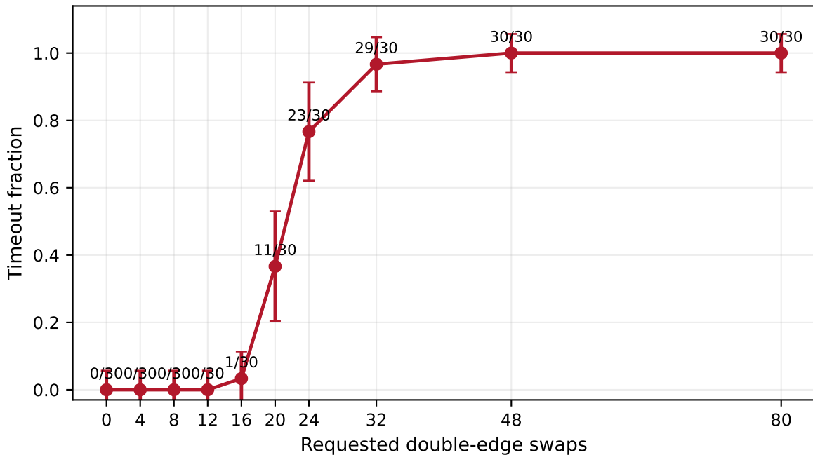
Kissat 4.0.4, 60 s limit; Wilson 95% intervals
