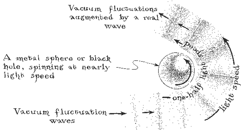
12.1 Zel'dovich's mechanism by which vacuum fluctuations cause a spinning body to radiate.
