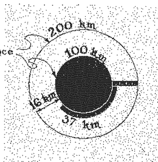
FLAT SPACETIME
