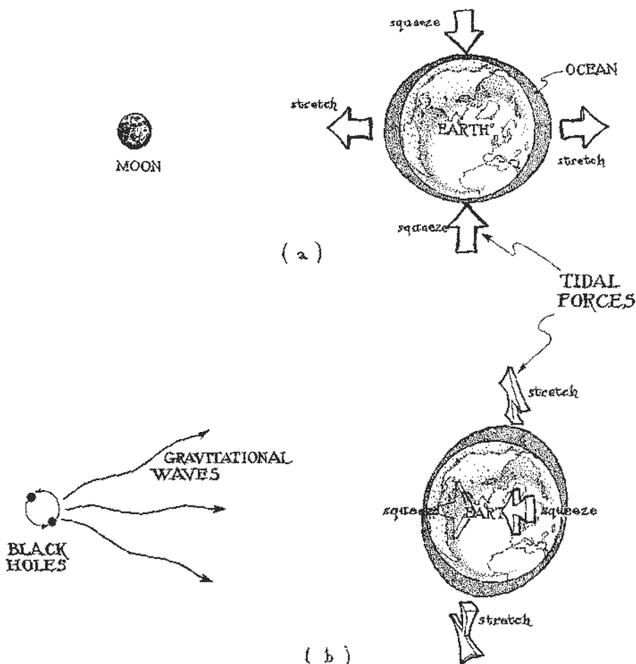
10.3 The tidal forces produced by the Moon and by a gravitational wave. (a) The Moon's tidal forces stretch and squeeze the Earth's oceans; the stretch is longitudinal, the squeeze is transverse. (b) A gravitational wave's tidal forces stretch and squeeze the Earth's oceans; the forces are entirely transverse, with a stretch along one transverse direction and a squeeze along the other.
