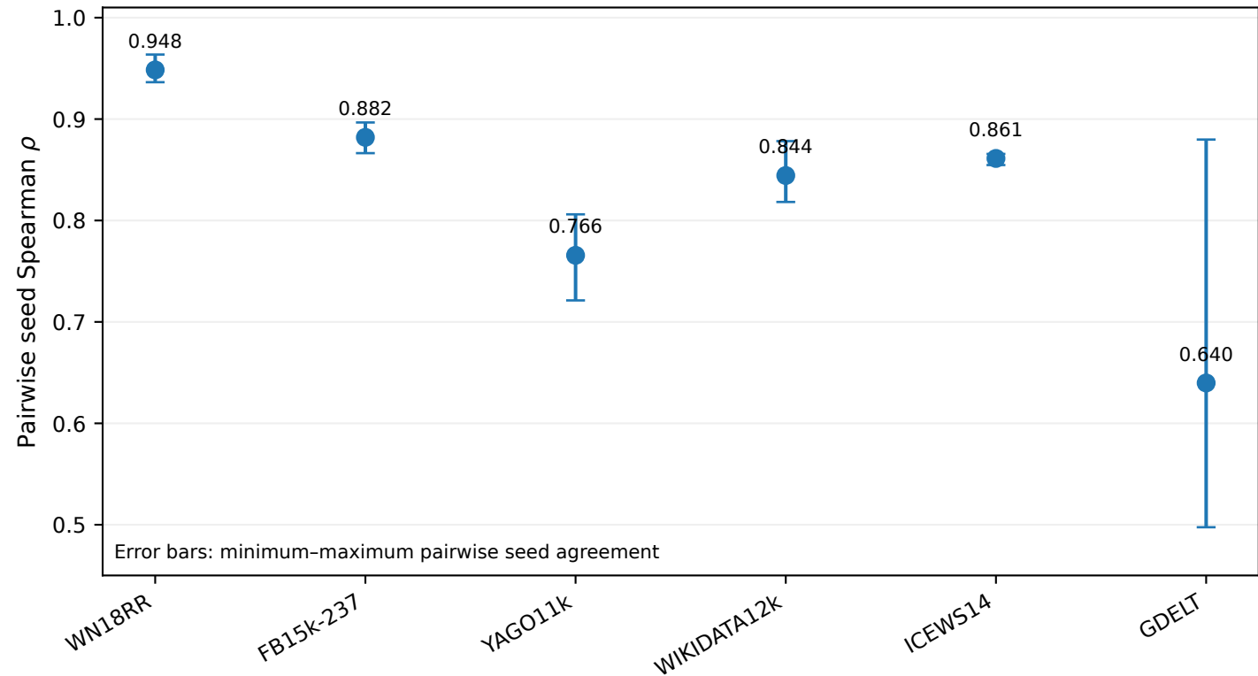
Learned curvature is reproducible across random seeds
