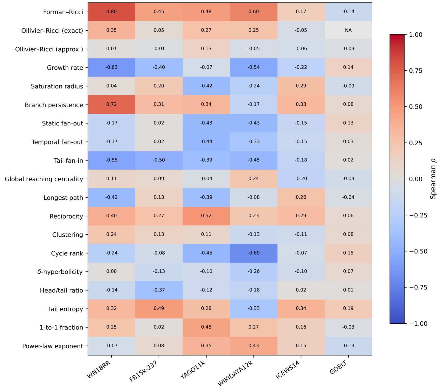
Structural correlates of learned relation-specific curvature
