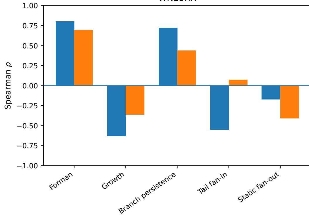
WN18RR
