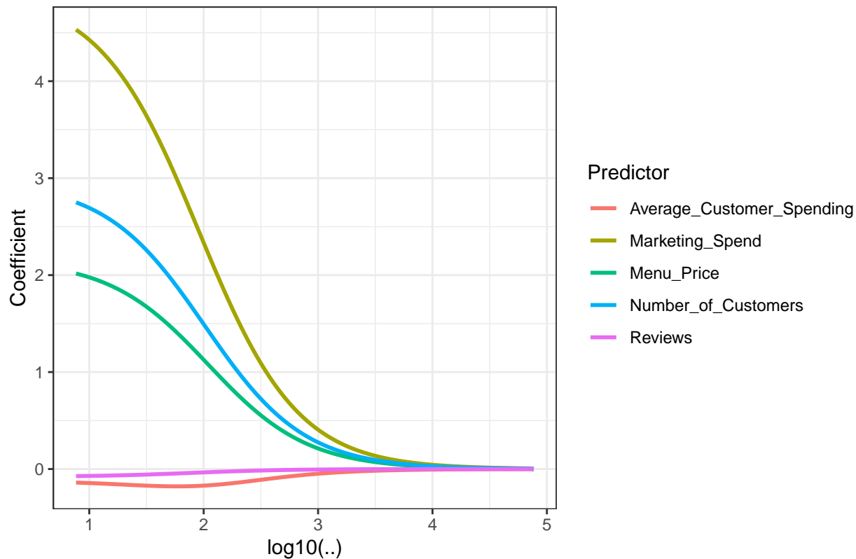
Ridge Coefficient Paths
