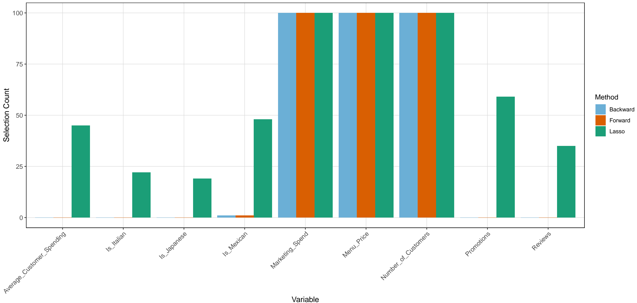
Selection Frequency (out of 100) for Each Variable
