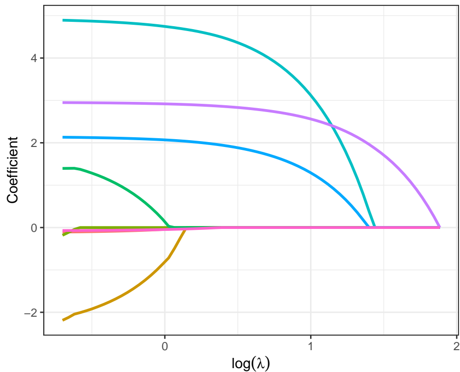
B. Lasso Coefficient Paths
