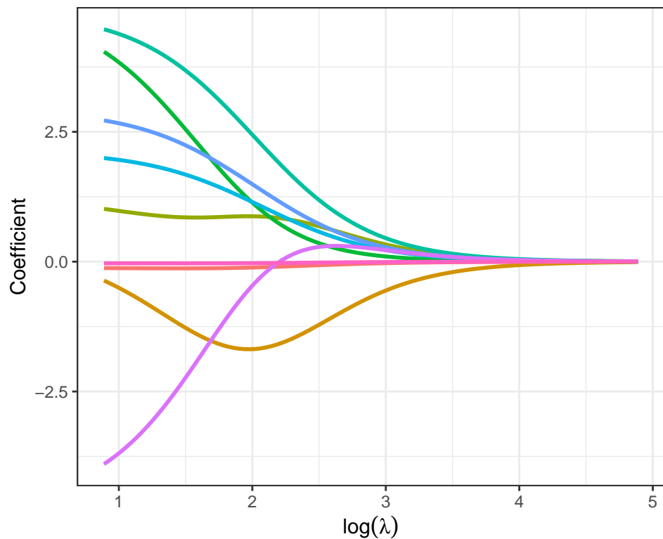
A. Ridge Coefficient Paths
