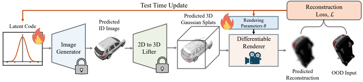
Figure 3: Analysis-by-synthesis inference paradigm. To handle OOD inputs, we employ a test-time optimization loop (red arrow). We freeze the Image Generator and 2D to 3D Lifter (indicated by lock icons) to preserve the learned prior. Instead, we optimize the Latent Code and Rendering Parameters (indicated by flame icons) to minimize the reconstruction loss \mathcal{L} between the rendered reconstruction and the OOD input. This ensures the input to the lifter remains a valid predicted ID image while matching the OOD observation.
