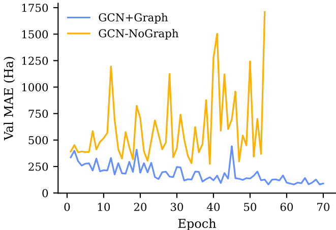
Learning Curves: Graph vs. No Graph
