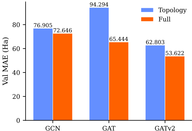
Topology vs. Full Node Features
