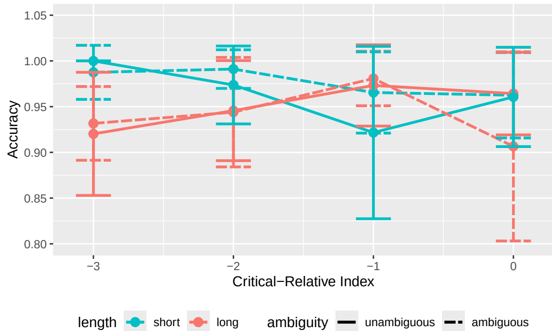
Accuracy by Critical-Relative Index ( final items)
