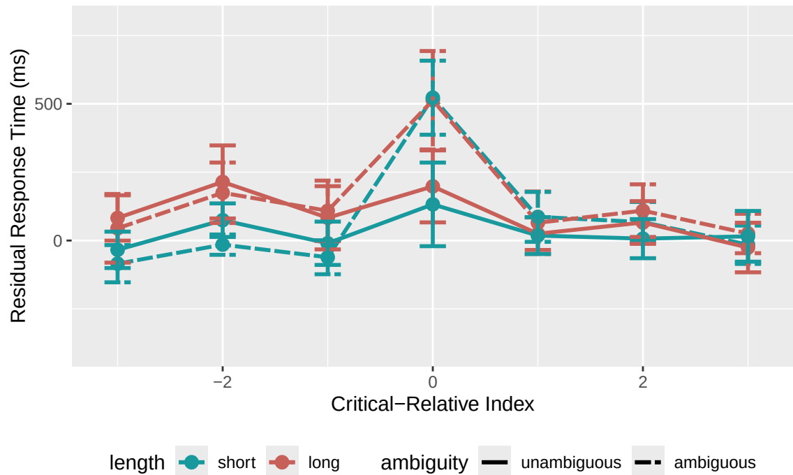
Residual RTs by Critical-Relative Index (nonfinal items)
