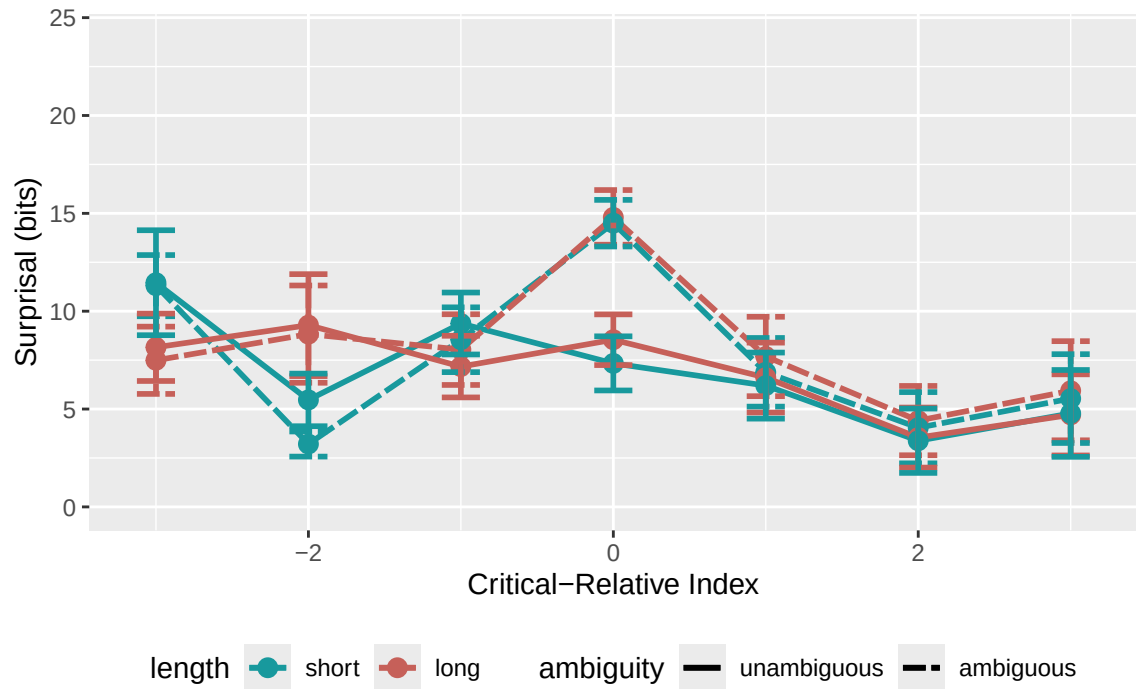
LLM Surprisal by Critical-Relative Index (nonfinal items)
