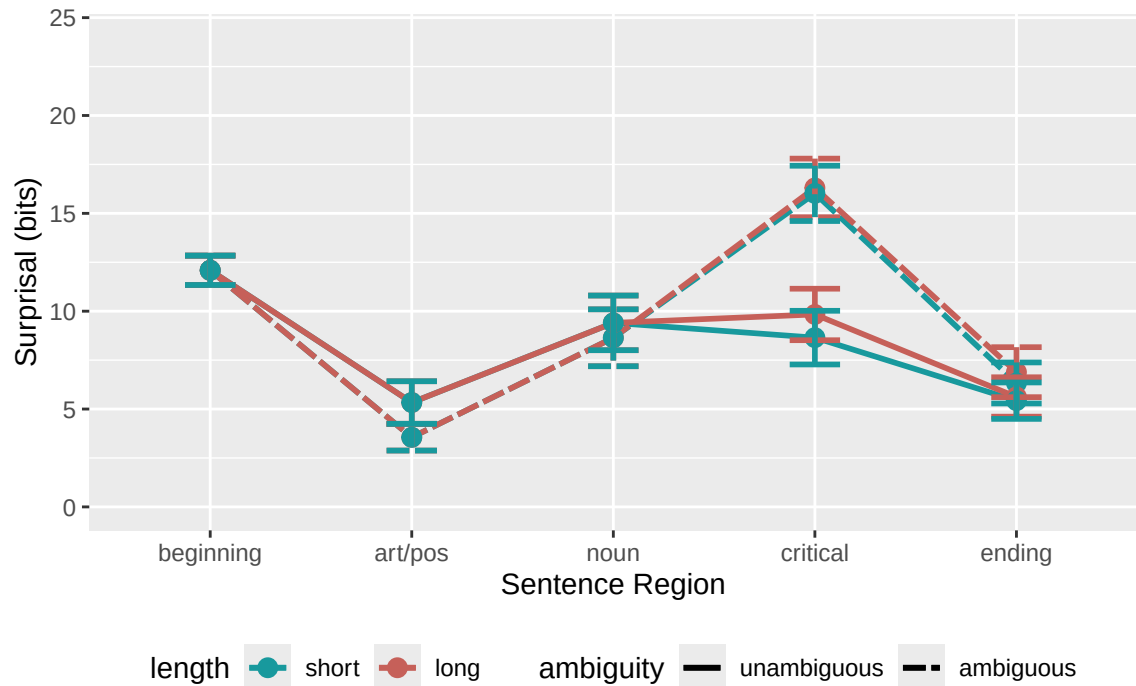
LLM Surprisal by Sentence Region (all items)
